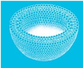
Diagram of catezome structure
